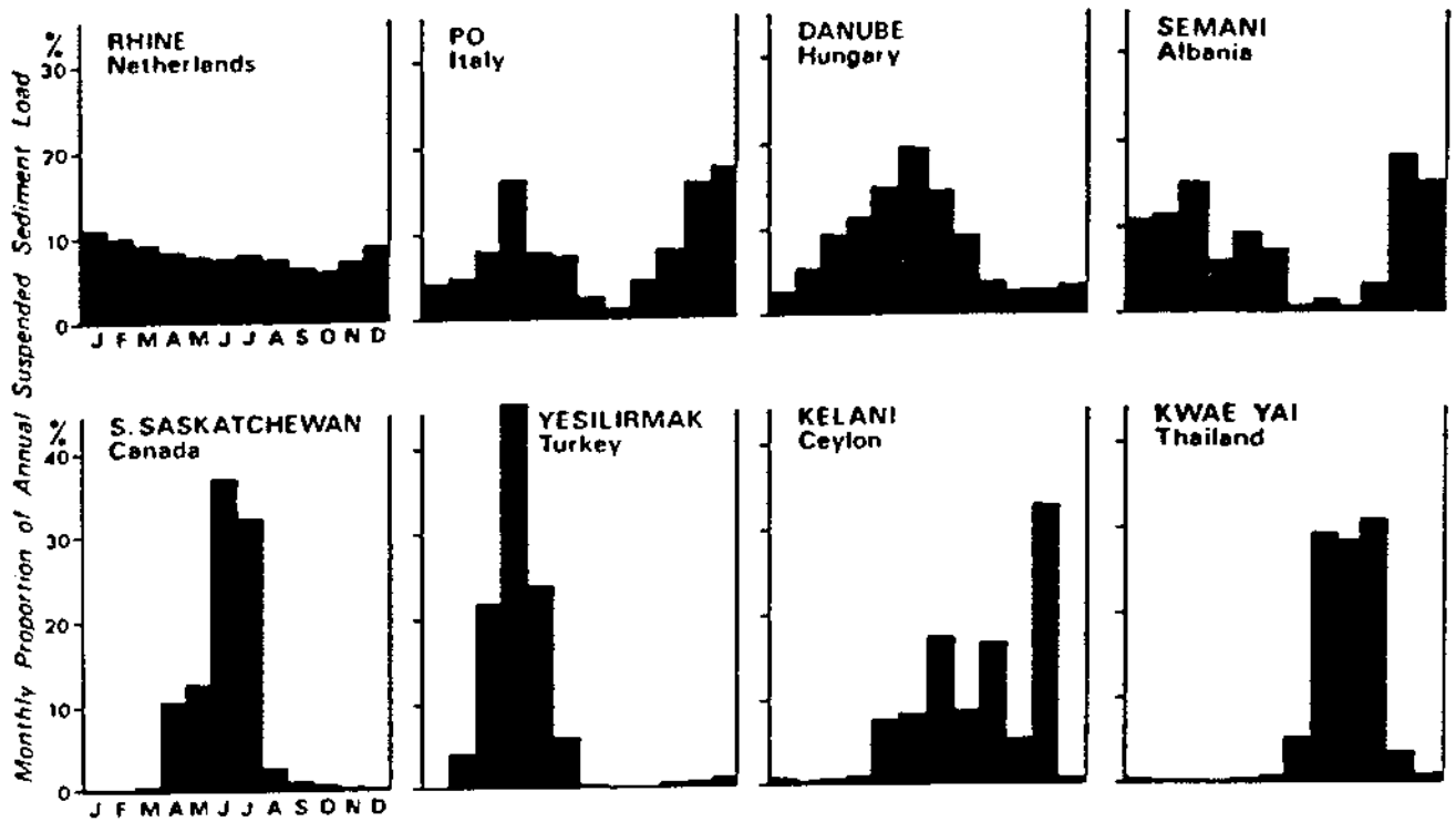
Figure A.V-5. Selected suspended sediment regimes (after Gregory and Walling, 1973).
