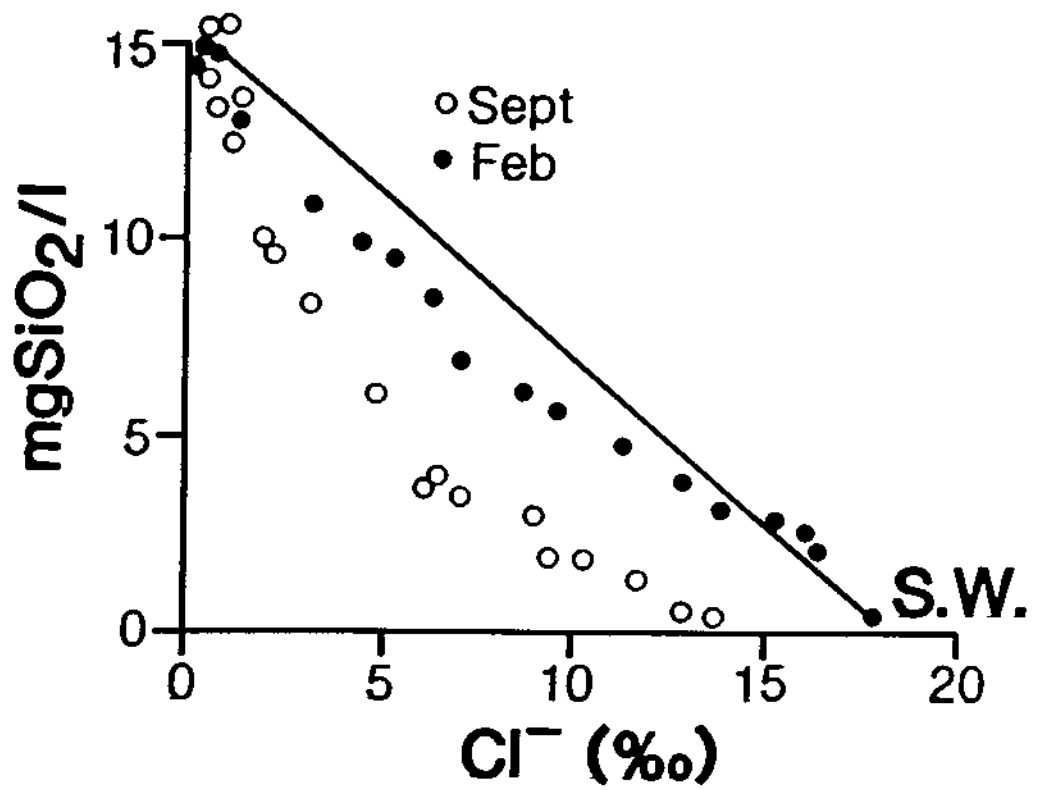
Figure A.II-3. Relationships between dissolved silica and salinity in the Scheldt estuary observed in February and September. Conservative mixing is represented by the straight line. (Wollast, R. and Beckers, O., unpublished data.)
