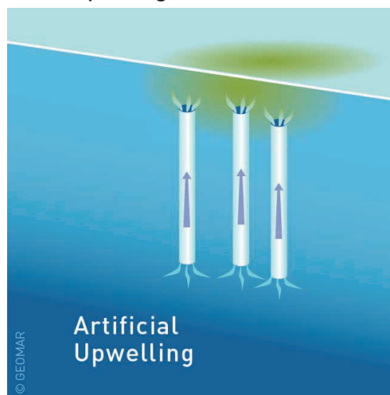
Figure 5.12 Artificial upwelling
